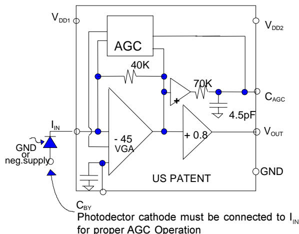
Figure 1: Equivalent Circuit
