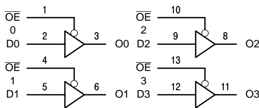
Figure 2. Logic Diagram
