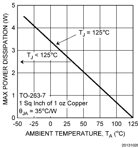
FIGURE 4. Maximum Power Dissipation vs Ambient Temperature for the TO-263 Package
