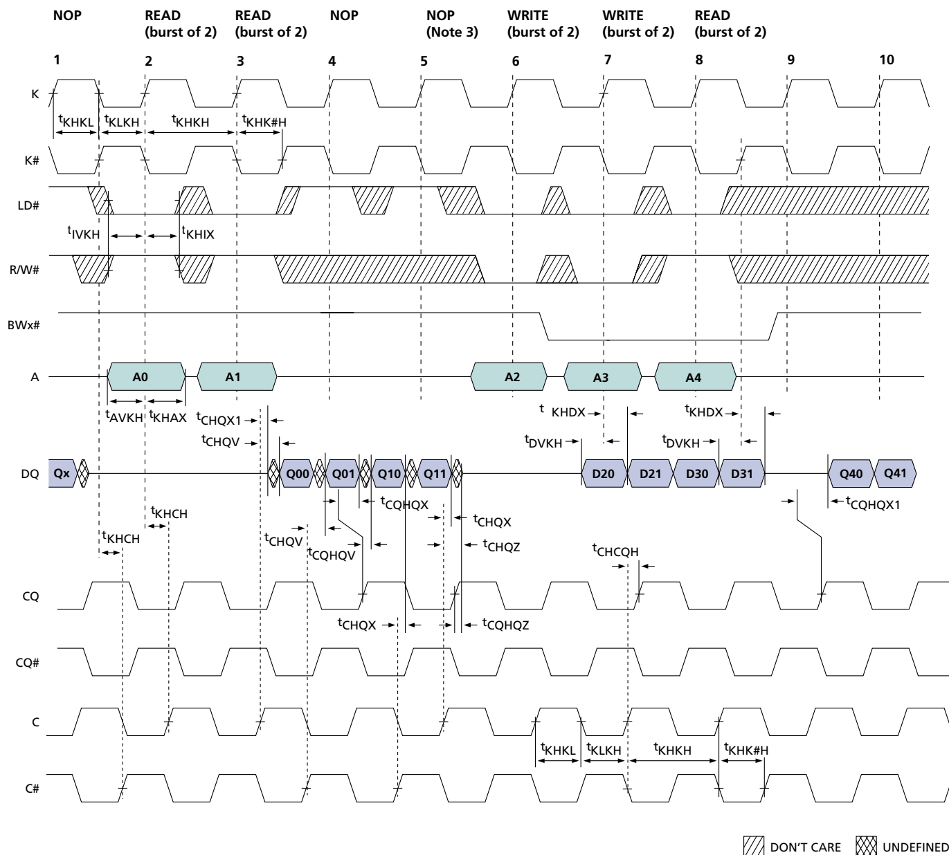
Figure 6: READ/WRITE Timing
