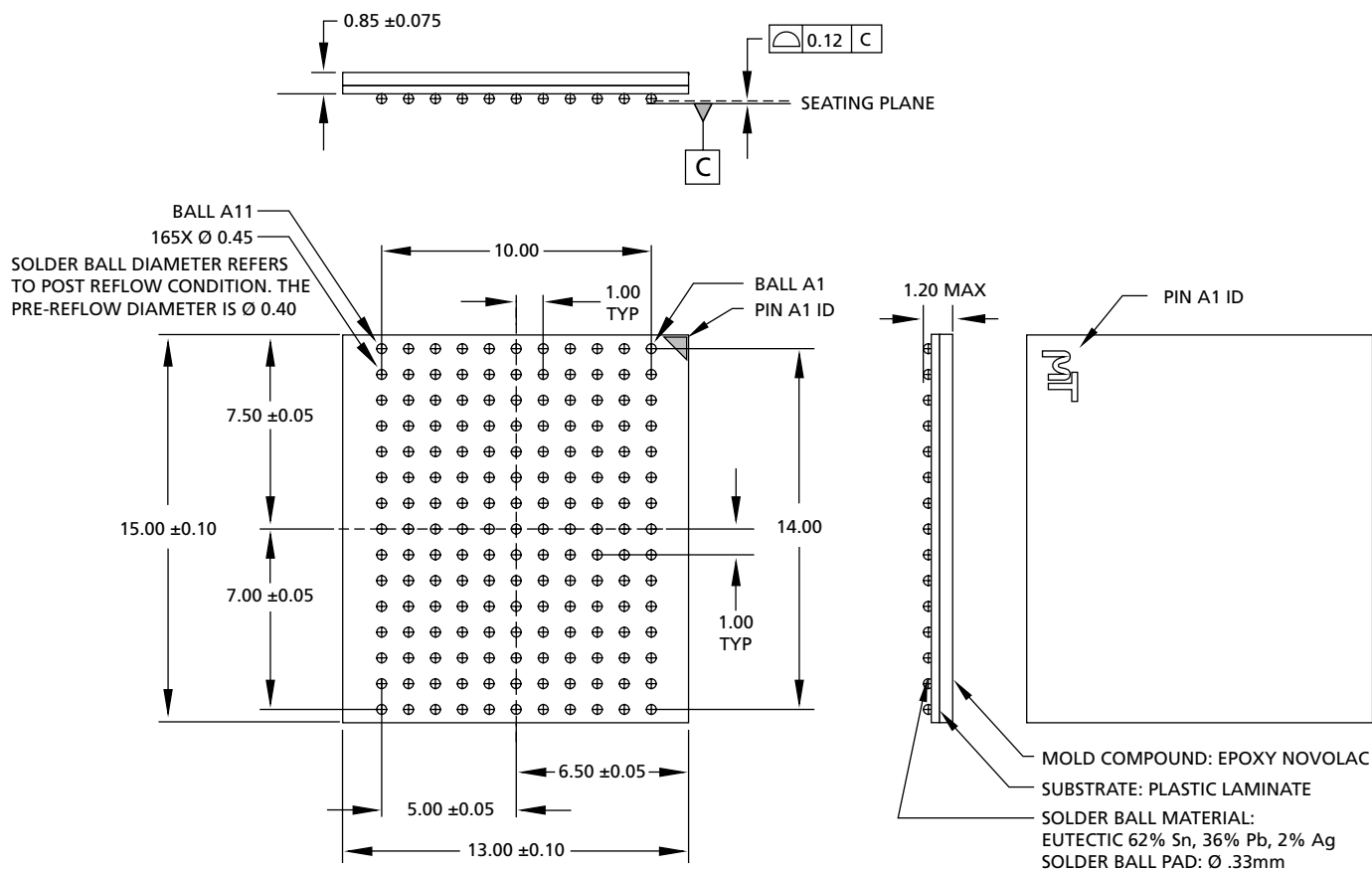
Figure 11: 165-Ball FBGA
