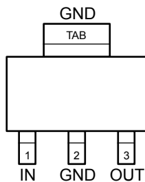
SOT-223 (S) MIC37100-x.x (Fixed)
