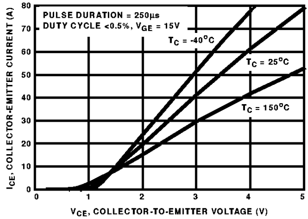
FIGURE 4. COLLECTOR-EMITTER ON-STATE VOLTAGE
