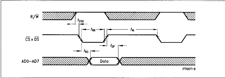
Figure 39 μP Read Cycle
