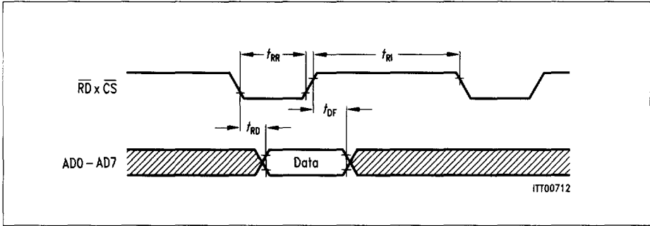
Figure 35 \mu P Write Cycle
