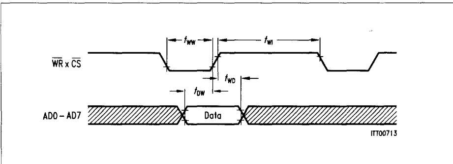
Figure 36 \mu P Write Cycle
