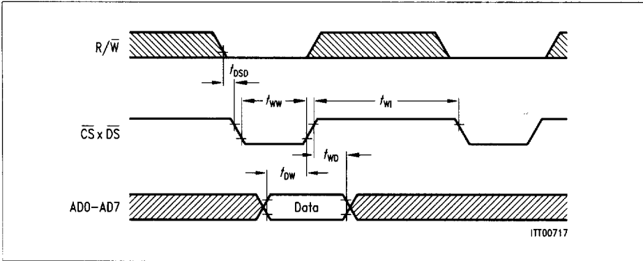
Figure 40 μP Write Cycle
