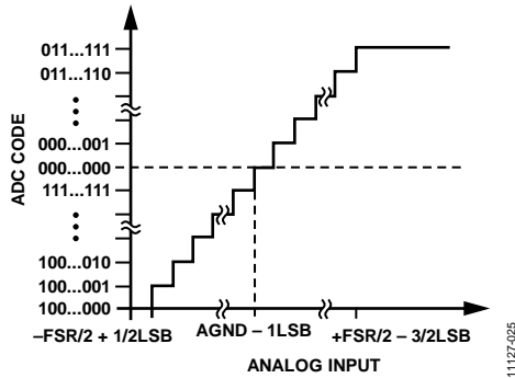
Figure 21. Transfer Characteristic
