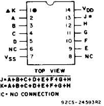
TERMINAL ASSIGNMENT
