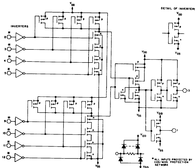
Fig. 8 - Schematic diagram.
