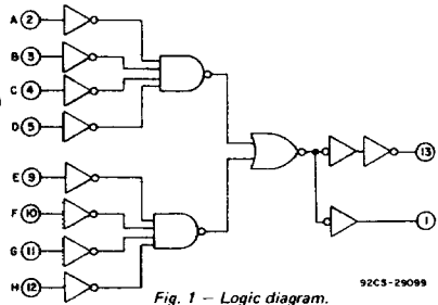
Fig. 1 - Logic diagram.
