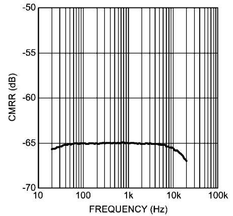
CMRR vs Frequency V_{DD} = 3.3V, V_{CM} = 1V_{P-P}, R_L = 8\Omega Earpiece Bypass Mode
