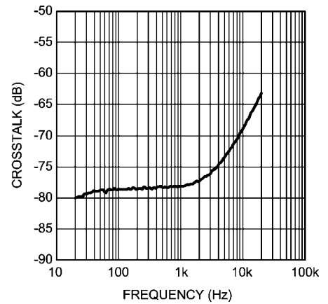
Crosstalk vs Frequency V_{DD} = 3.3V, V_{CM} = 1V_{P-P}, R_L = 32\Omega Headphone Mode 8
