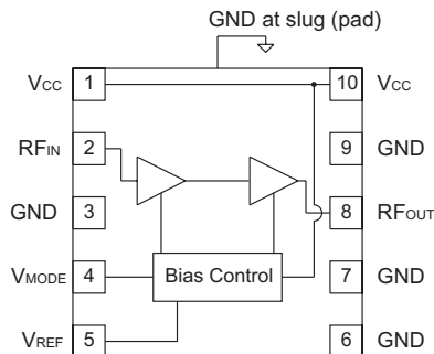
Figure 1: Block Diagram
