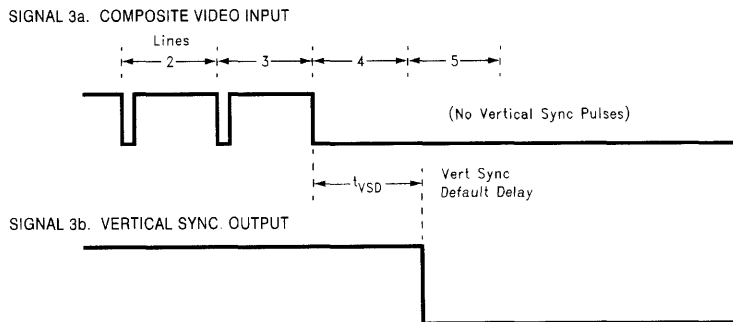
Figure 3. Non-Standard Vertical Timing
