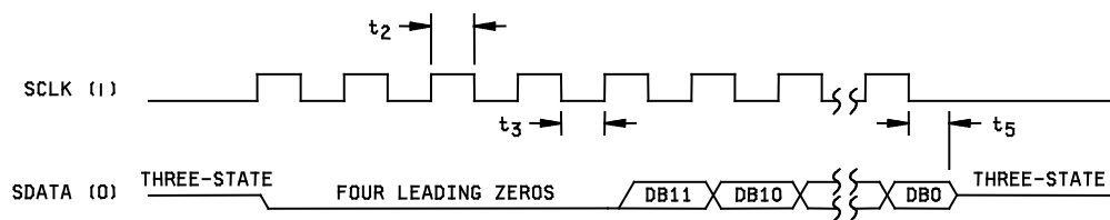
DATA READ OPERATION
