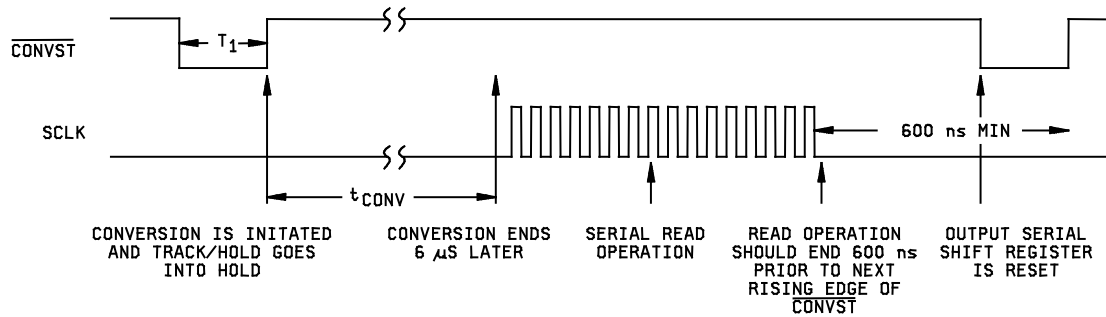
TIMING SEQUENCE FOR OPTIMUM PERFORMANCE
