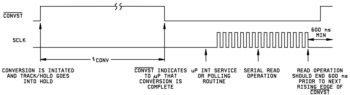
CONVST USED AS STATUS SIGNAL
