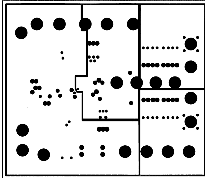
FIGURE 20. Internal Plane 2
