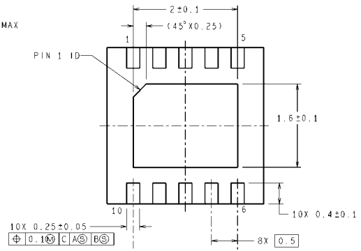
LLP, 10 Lead, Package NS Package Number SDA10A
