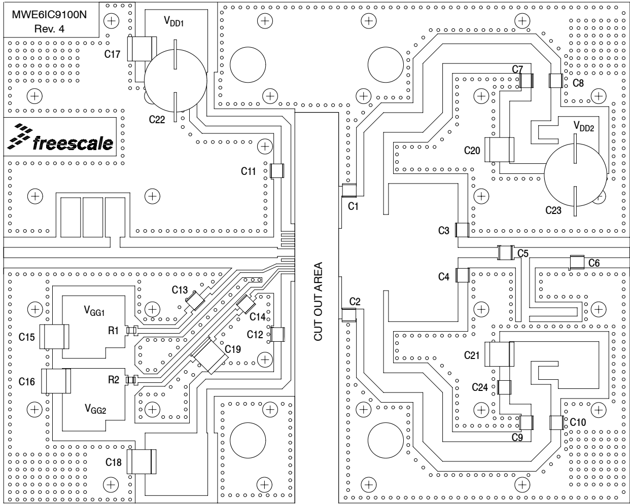
Figure 4. MWE6IC9100NR1 Test Circuit Component Layout
