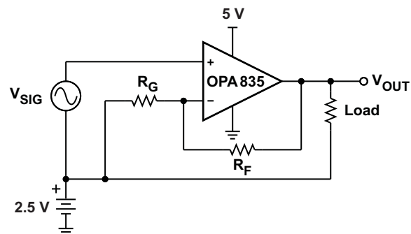
Figure 59. Single-Supply Concept
