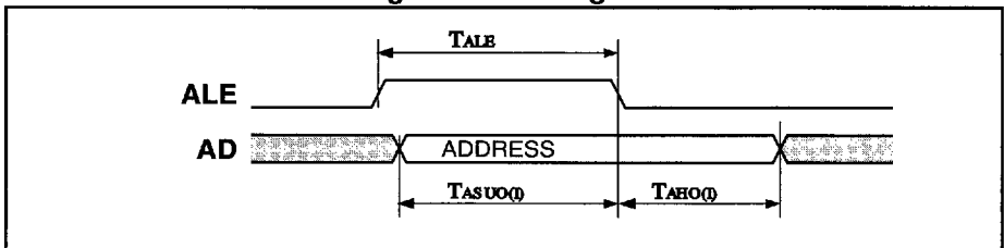
Figure 4: ALE Signal
