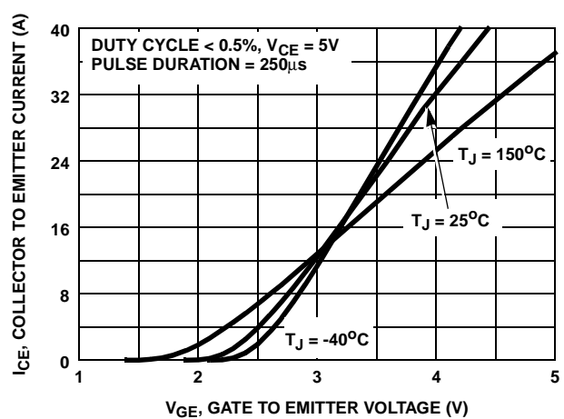
FIGURE 10. TRANSFER CHARACTERISTIC
