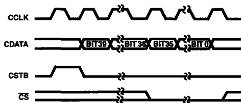
FIGURE 14. CONTROL WORD TIMING DIAGRAM
