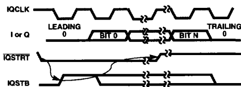
FIGURE 13. REQUESTED DATA OUTPUT TIMING
