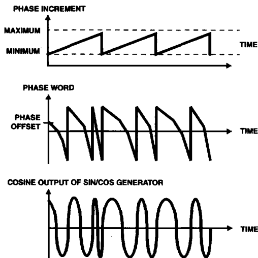
FIGURE 4B. UP CHIRP
