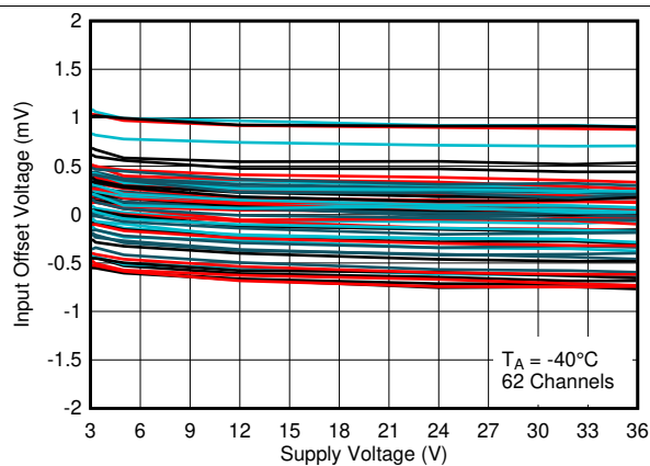
Figure 17. Input Offset Voltage vs. Supply Voltage at -40^\circ\text{C}
