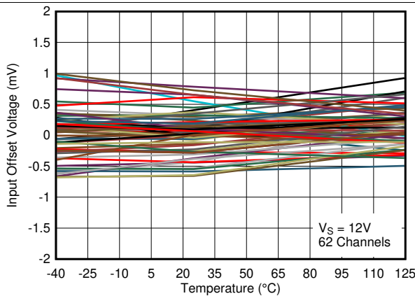
Figure 15. Input Offset Voltage vs. Temperature at 12V
