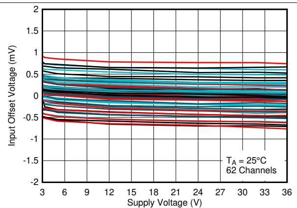
Figure 18. Input Offset Voltage vs. Supply Voltage at 25^\circ\text{C}
