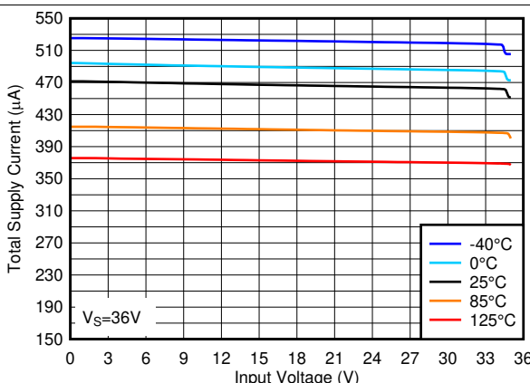
Figure 12. Total Supply Current vs. Input Voltage at 36V
