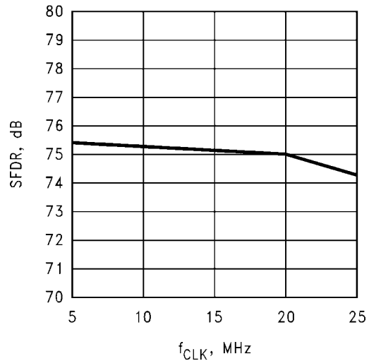
SFDR vs. f_{CLK} @ f_{IN} = 9.5 MHz
