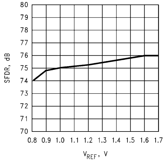
SFDR vs. V_{REF} @ f_{IN} = 4.7 MHz
