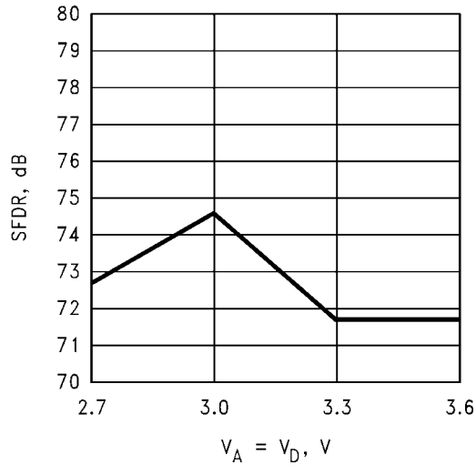
SFDR vs. Supply Voltage @ f_{IN} = 4.7 MHz
