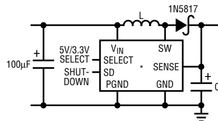
Figure 3. Basic Step-Up Converter
