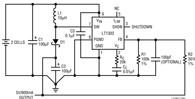
Figure 5. LT1302 High Current Step-Up from 2 Cells
