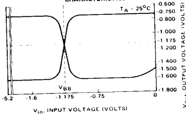
FIGURE 8 - A/D COMPARATOR
