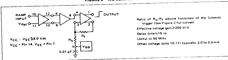
FIGURE 8 - A/D COMPARATOR
