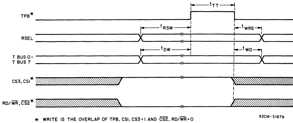
Fig. 5 - Mode 1 CPU interface (WRITE) timing diagram.
