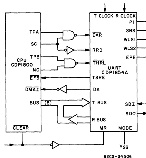
Fig. 8 - Mode 0 connection diagram.
