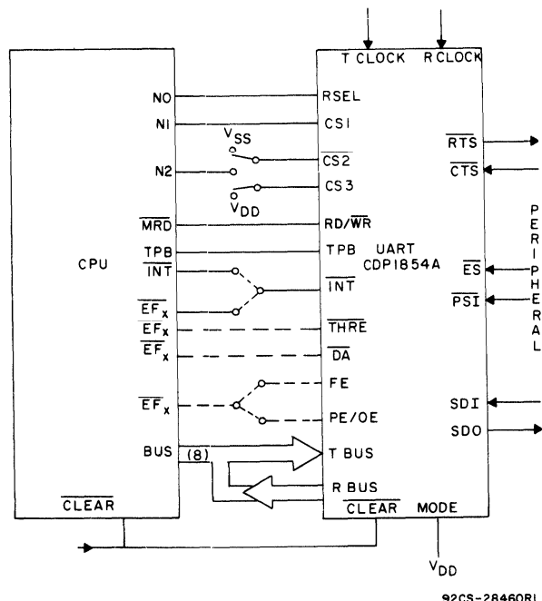
Fig. 2 - Recommended CDP1800-series connection, Mode 1 (non-interrupt driven system).
