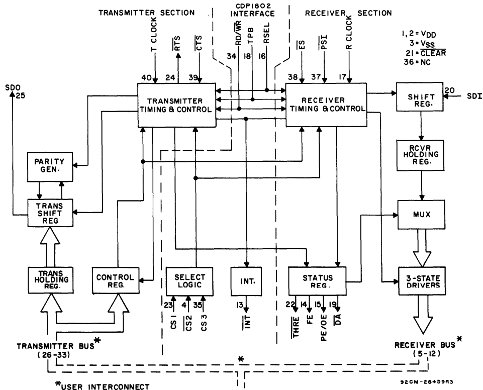
Fig. 1 - Mode 1 block diagram (CDP1800-series microprocessor compatible).
