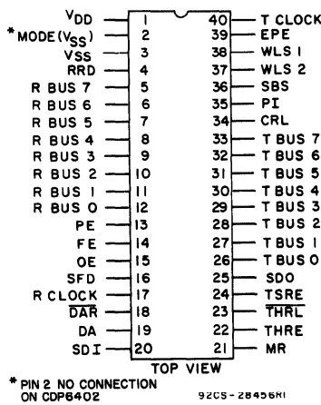
Mode 0 Terminal Assignment
