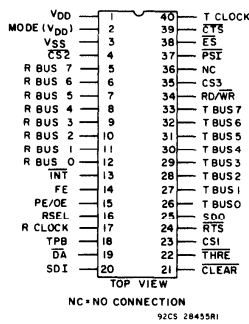
Mode 1 Terminal Assignment
