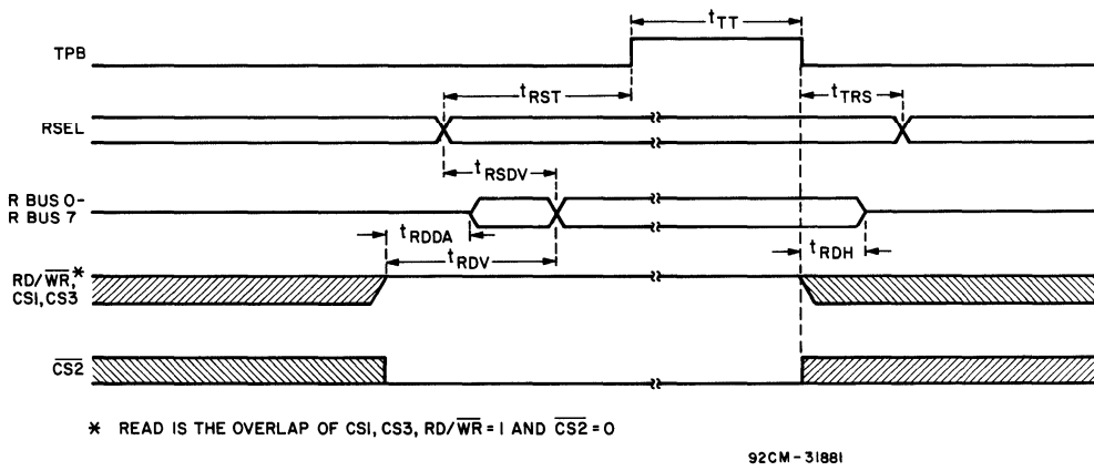
Fig. 6 - Mode 1 CPU interface (READ) timing diagram.
