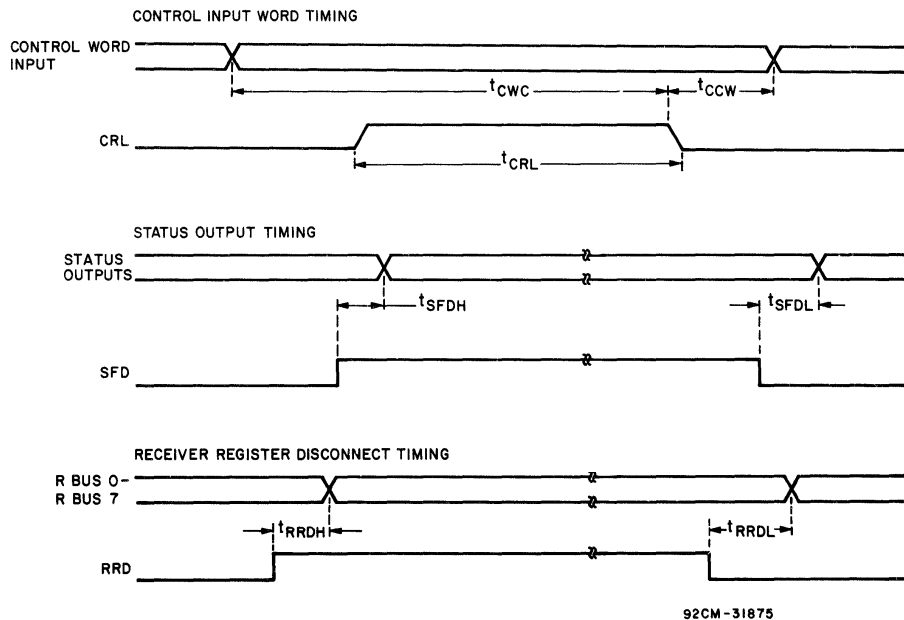
Fig. 9 - Mode 0 interface timing diagram.
