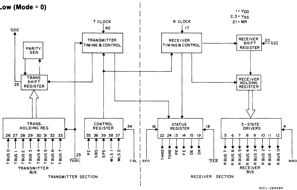
Fig. 7 - Mode 0 block diagram (industry standard compatible).
