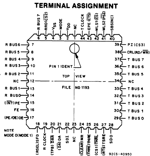
44-Lead Plastic Chip-Carrier Package (Q Suffix)
