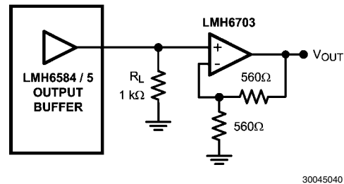
FIGURE 12. Buffered Output
