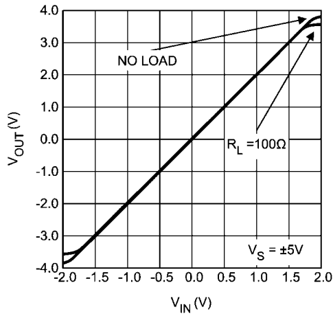
Output Swing
