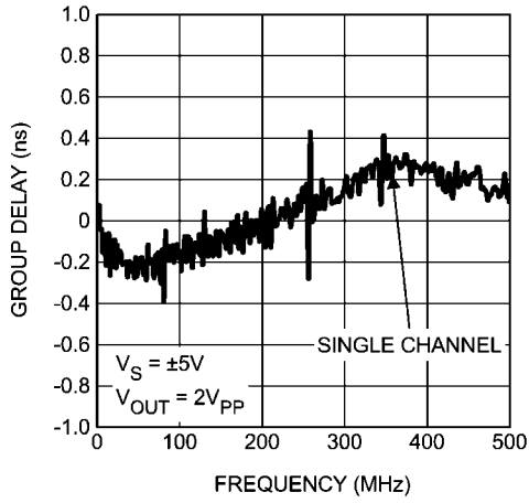
Group Delay
