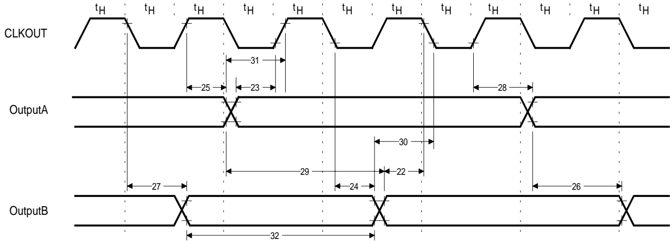
Figure 112. General Output Timing
