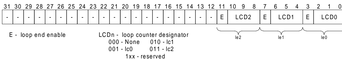
Figure 29. lctl Register
