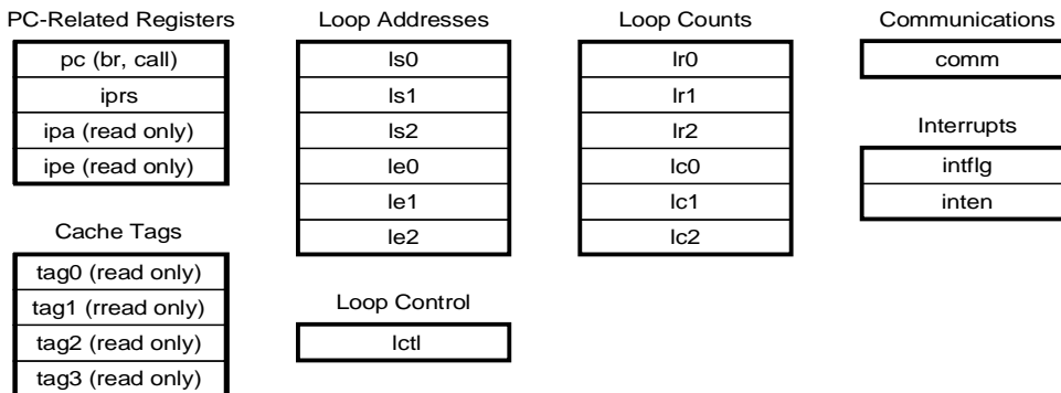
Figure 23. PP Registers
