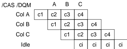
Burst length 1, 3 cycle latency (CT = 1001) reads, read transfers, split-read transfers
