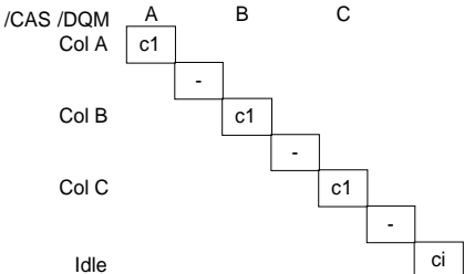
Burst length 2 block writes
