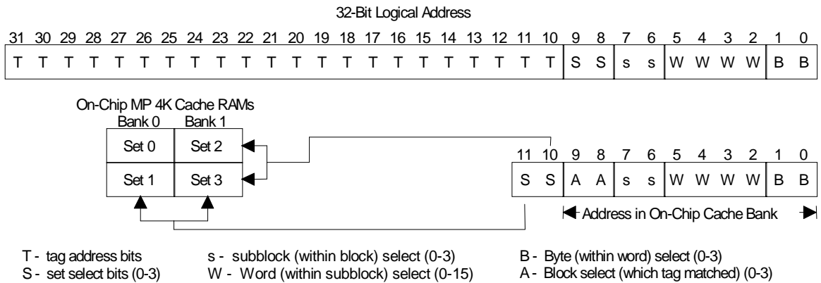
Figure 19. Cache Addressing
