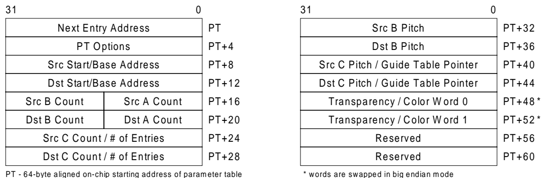
Figure 52. Packet Transfer Parameter Table - Long Form
