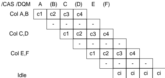
Burst length 2, 3 cycle latency (CT = 1101) reads, read transfers, split-read transfers
