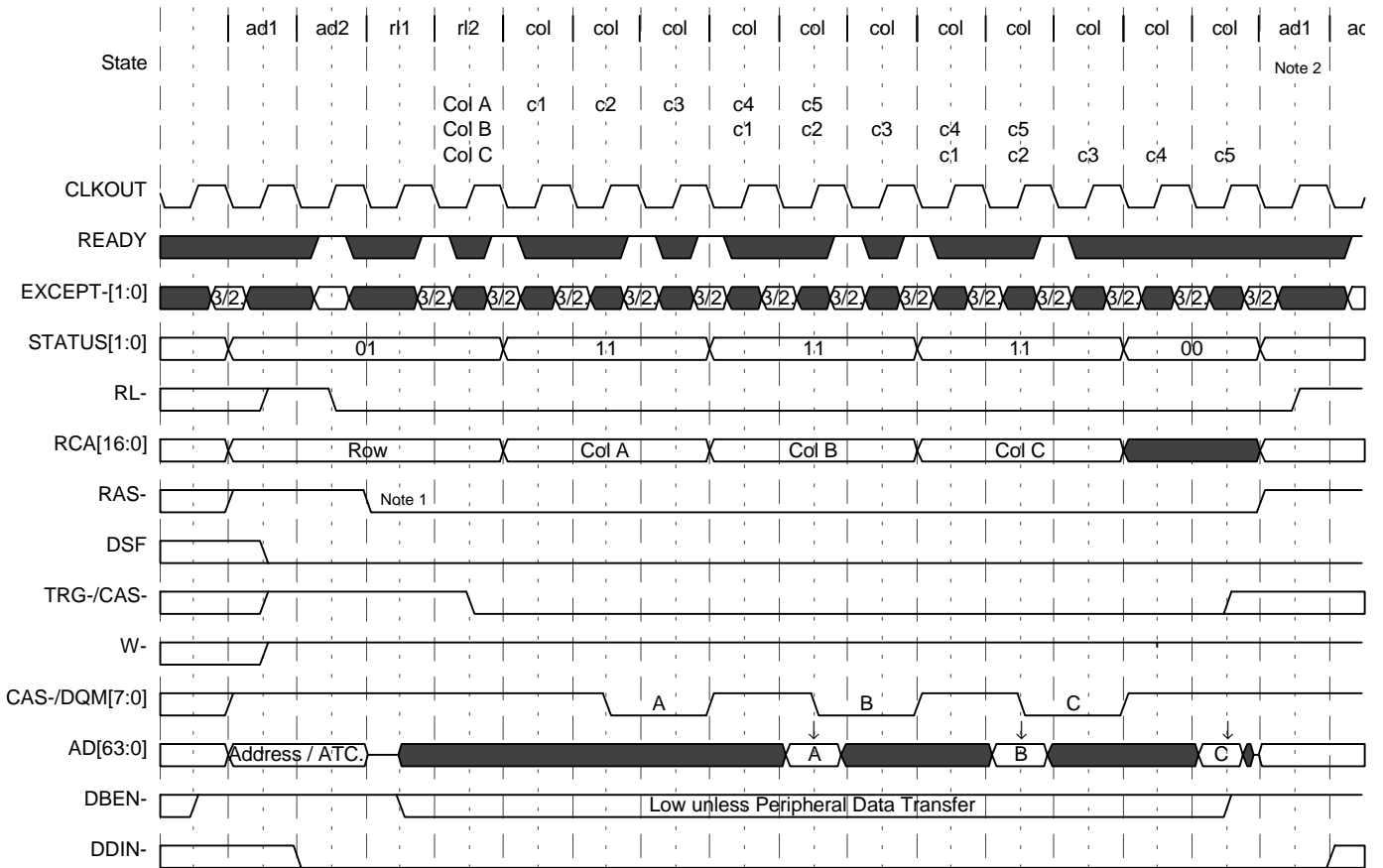
Figure 63. 3 cycle/column EDO DRAM Read Cycle
