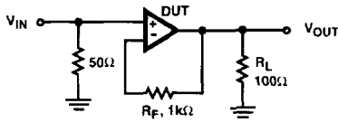
FIGURE 2. SMALL SIGNAL PULSE RESPONSE CIRCUIT
