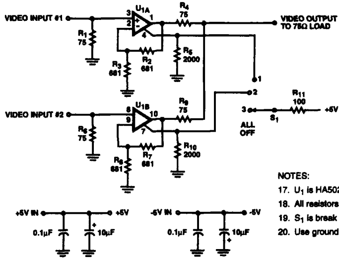
FIGURE 9. TWO CHANNEL HIGH IMPEDANCE MULTIPLEXER
