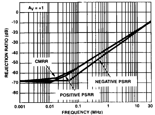
FIGURE 22. REJECTION RATIOS vs FREQUENCY
