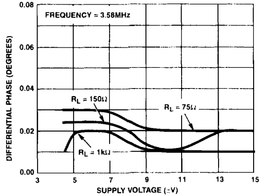
FIGURE 20. DIFFERENTIAL PHASE vs SUPPLY VOLTAGE
