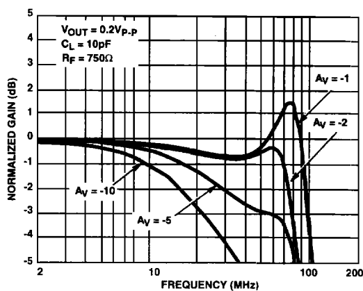
FIGURE 12. INVERTING FREQUENCY RESPONSE
