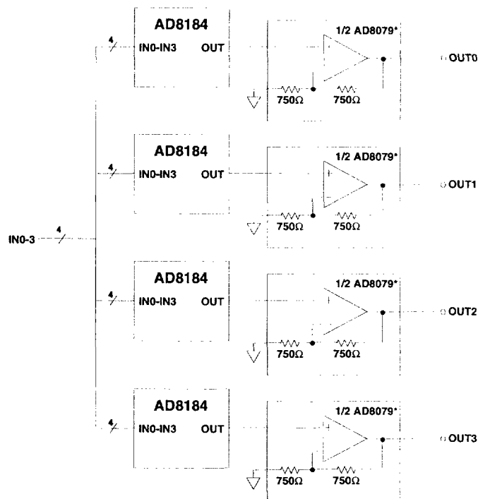
Figure 24. 4 × 4 Crosspoint Switch
