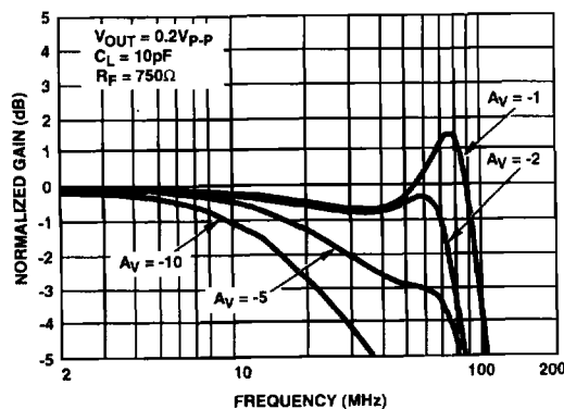
FIGURE 9. INVERTING FREQUENCY RESPONSE
