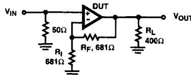
FIGURE 3. LARGE SIGNAL PULSE RESPONSE CIRCUIT
