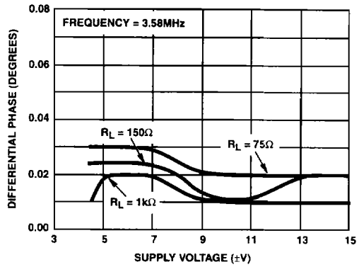
FIGURE 17. DIFFERENTIAL PHASE vs SUPPLY VOLTAGE
