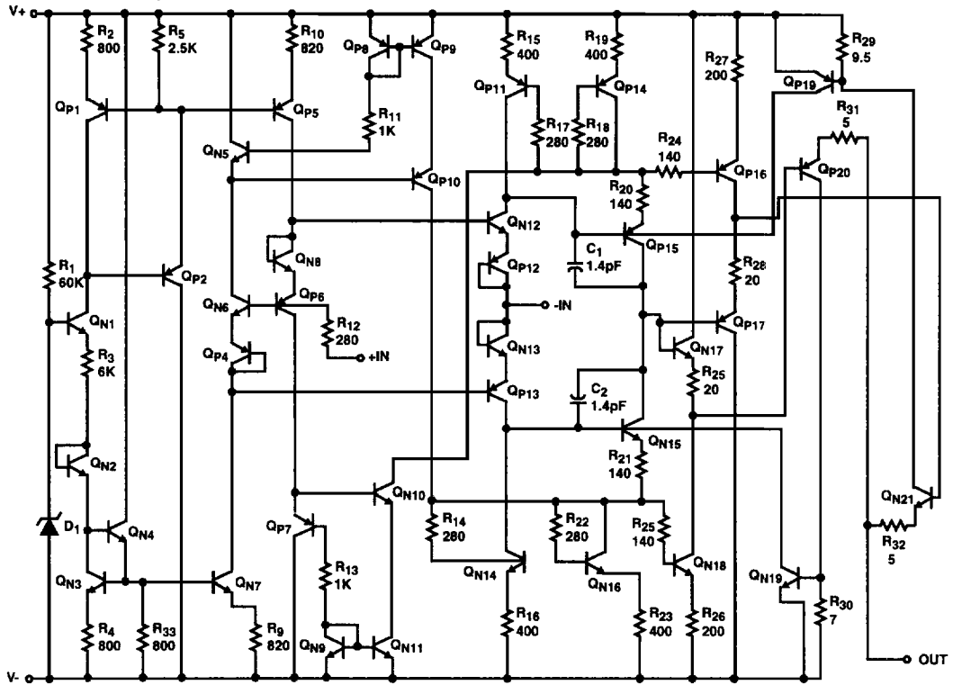
Schematic Diagram (One Amplifier of Four)
