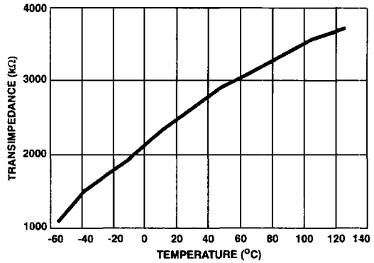
FIGURE 29. TRANSMIMPEDANCE vs TEMPERATURE
