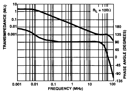
FIGURE 39. TRANSIMPEDANCE vs FREQUENCY
