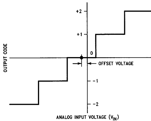
FIGURE 6. Offset or Zero Error Voltage
