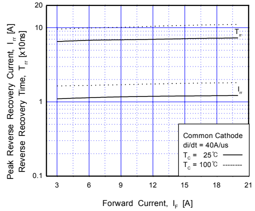
Fig 16. Reverse Recovery Characteristics
