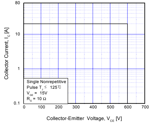
Fig 14. RBSOA Characteristics
