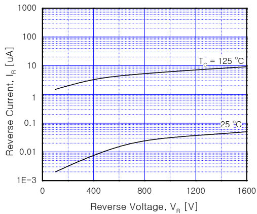
Fig 17. Rectifier (Converter) Characteristics
