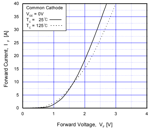
Fig 15. Forward Characteristics
